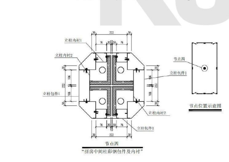
Partition wall intermediate column color steel components and lining
