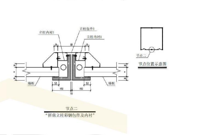
Partition wall column color steel components & lining
